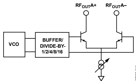
Figure 22. Output Stage
