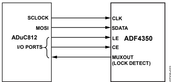
Figure 35. ADuC812 to ADF4350 Interface
