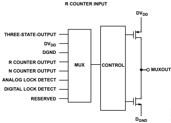
Figure 19. MUXOUT Schematic
